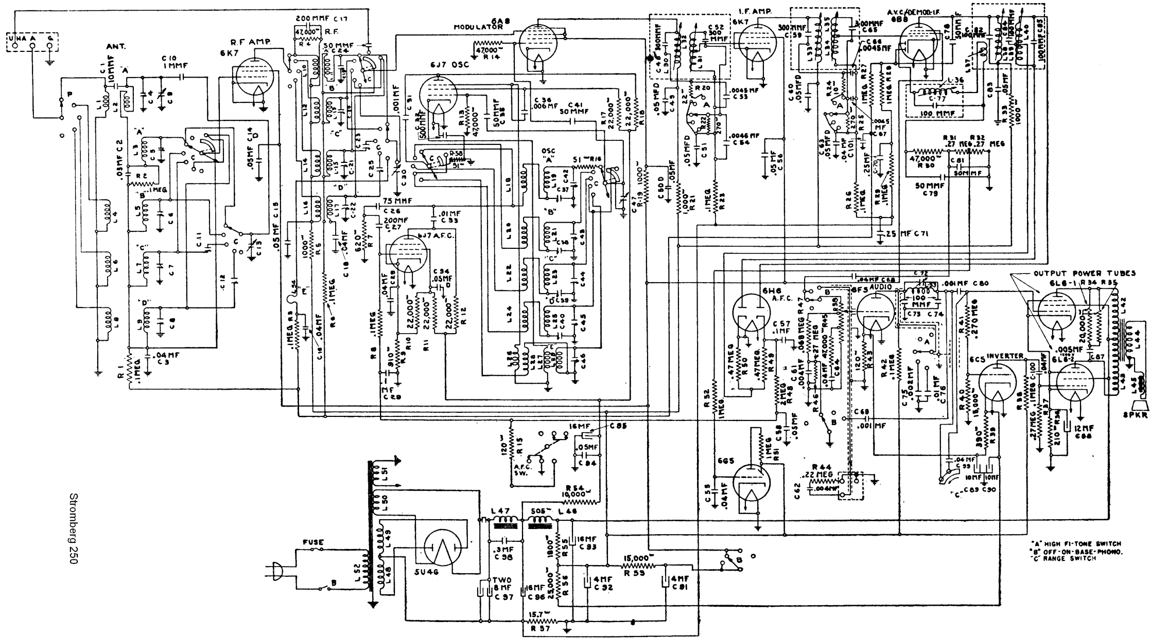
Fig. 2. Schematic Circuit.
